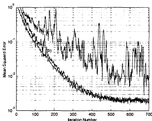
Fig. 5. Comparison results of (a) LMS, (b) modified DLMS using optimized tree, and (c) conventional DLMS.
